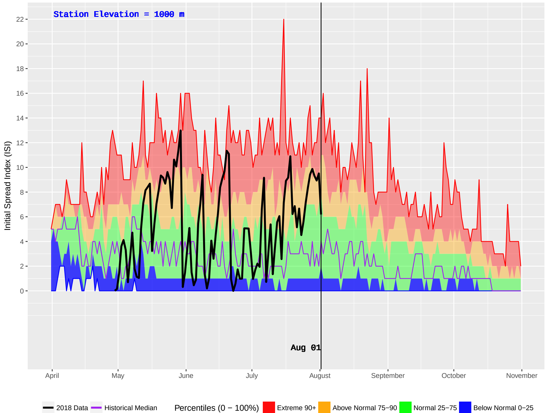
SUCCOUR CREEK (374) : Historical (1986–2016) and Current (2018) Daily Initial Spread Index (ISI)
