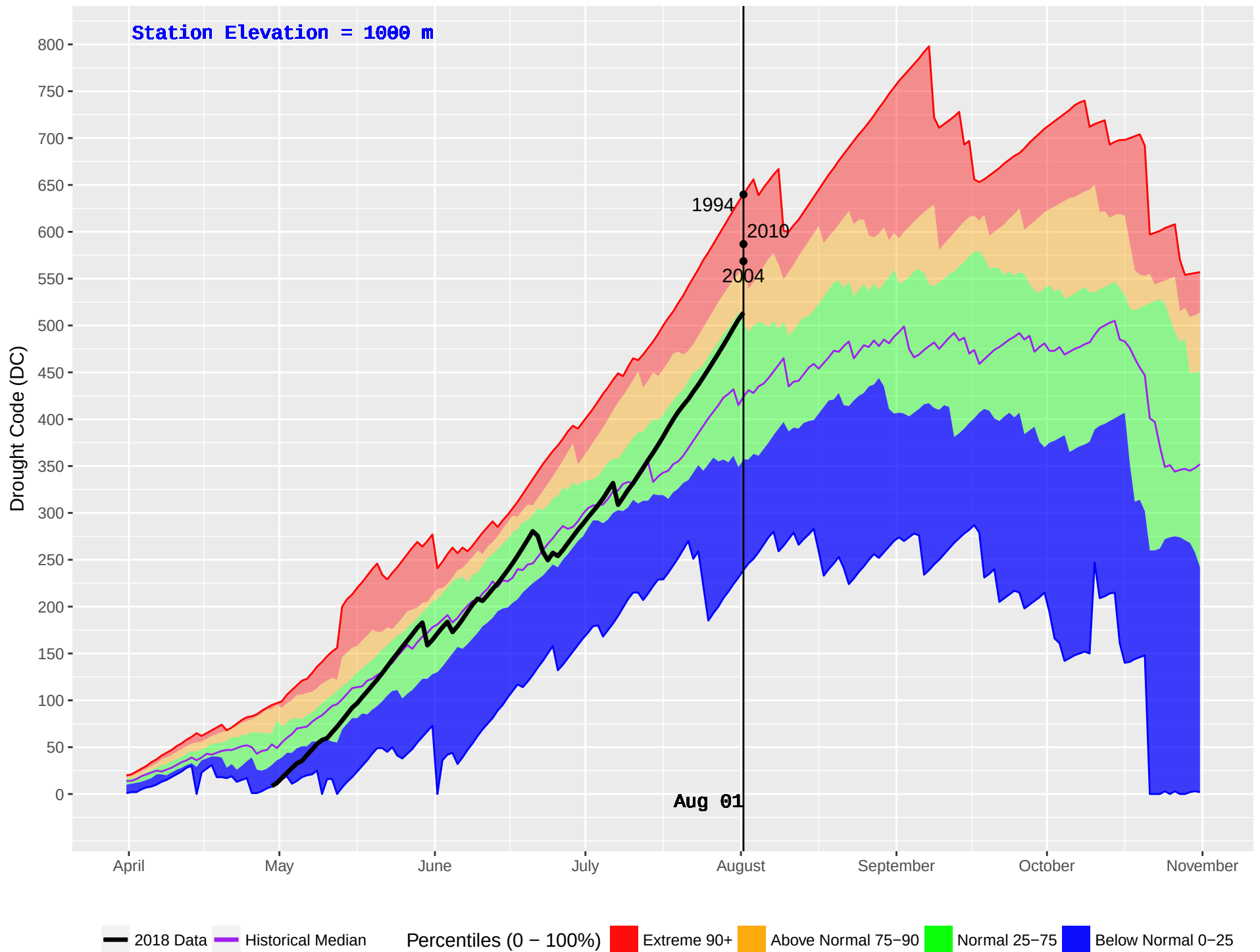
SUCCOUR CREEK (374) : Historical (1986–2016) and Current (2018) Daily Drought Code (DC)
